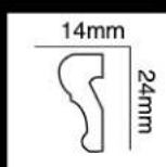
HG-8506 长度(Long):2400mm 面宽(Breath):24mm
