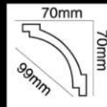
HG-9547 长度(Long):2400mm 面宽(Breath):99mm
