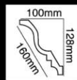
HG-9612 长度(Long):2400mm 面宽(Breath):160mm
