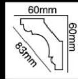
HG-7510 长度(Long):2400mm 面宽(Breath):83mm
