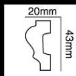
HG-8531 长度(Long):2400mm 面宽(Breath):43mm
