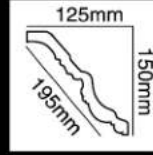
HG-7671 长度(Long):2400mm 面宽(Breath):195mm
