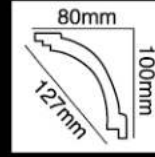
HG-9597 长度(Long):2400mm 面宽(Breath):127mm
