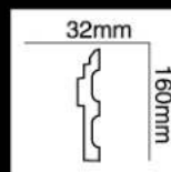
HG-8601 长度(Long):2400mm 面宽(Breath):160mm
