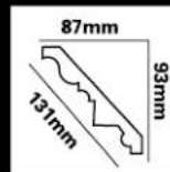
HG-9576 长度(Long):2400mm 面宽(Breath):131mm
