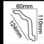
HG-7631 长度(Long):2400mm 面宽(Breath):124mm
