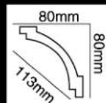
HG-9566 长度(Long):2400mm 面宽(Breath):113mm
