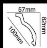
HG-7573 长度(Long):2400mm 面宽(Breath):100mm
