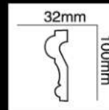
HG-8586 长度(Long):2400mm 面宽(Breath):100mm
