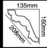
HG-7677 长度(Long):2400mm 面宽(Breath):208mm
