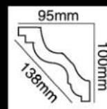
HG-9586 长度(Long):2400mm 面宽(Breath):138mm
