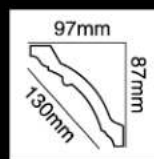
HG-7584 长度(Long):2400mm 面宽(Breath):130mm
