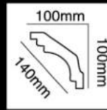
HG-7614 长度(Long):2400mm 面宽(Breath):140mm
