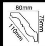
HG-7544 长度(Long):2400mm 面宽(Breath):110mm
