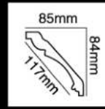
HG-7575 长度(Long):2400mm 面宽(Breath):117mm
