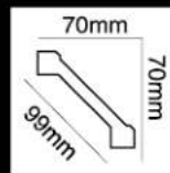
HG-9546 长度(Long):2400mm 面宽(Breath):99mm
