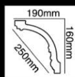
HG-7681 长度(Long):2400mm 面宽(Breath):250mm
