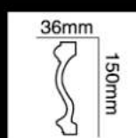
HG-8599 长度(Long):2400mm 面宽(Breath):150mm
