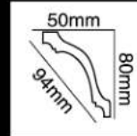
HG-9555 长度(Long):2400mm 面宽(Breath):94mm
