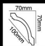
HG-7521 长度(Long):2400mm 面宽(Breath):100mm
