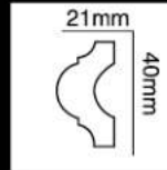
HG-6512 长度(Long):2400mm 面宽(Breath):40mm
