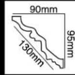
HG-7607 长度(Long):2400mm 面宽(Breath):130mm
