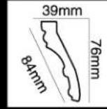
HG-7546 (水洗玫瑰銀) 長度 (Long) :2400 mm 面寬 (Breath) :84 mm 對花 (Pattern) :152 mm
