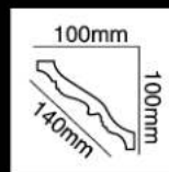
HG-7612 长度(Long):2400mm 面宽(Breath):140mm
