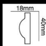
HG-8526 长度(Long):2400mm 面宽(Breath):40mm
