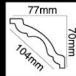
HG-9539 长度(Long):2400mm 面宽(Breath):104mm
