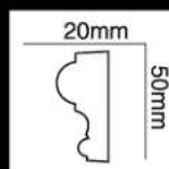
HG-8534 长度(Long):2400mm 面宽(Breath):50mm
