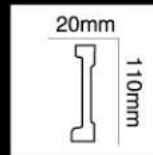
HG-6584 (仿紅木) 長度 (Long) :2400 mm 面寬 (Breath) :110 mm 對花 (Pattern) :203 mm
