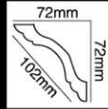
HG-9553 长度(Long):2400mm 面宽(Breath):102mm
