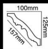
HG-7651 长度(Long):2400mm 面宽(Breath):157mm
