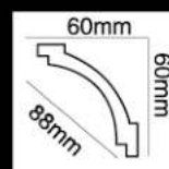
HG-9526 长度(Long):2400mm 面宽(Breath):88mm
