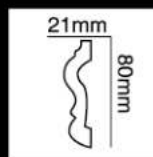
HG-8564 长度(Long):2400mm 面宽(Breath):80mm
