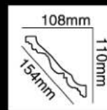
HG-7633 长度(Long):2400mm 面宽(Breath):154mm
