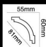
HG-9532 长度(Long):2400mm 面宽(Breath):81mm
