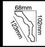
HG-7623 长度(Long):2400mm 面宽(Breath):123mm
