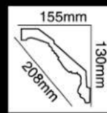
HG-7659 长度(Long):2400mm 面宽(Breath):208mm
