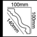
HG-9595 长度(Long):2400mm 面宽(Breath):140mm
