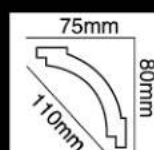
HG-9571 长度(Long):2400mm 面宽(Breath):110mm
