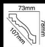
HG-7552 长度(Long):2400mm 面宽(Breath):107mm
