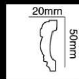
HG-6522 长度(Long):2400mm 面宽(Breath):50mm
