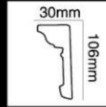
HG-6580 (仿古銅) 長度 (Long) :2400 mm 面寬 (Breath) :106 mm 對花 (Pattern) :237 mm
