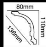
HG-7632 长度(Long):2400mm 面宽(Breath):136mm
