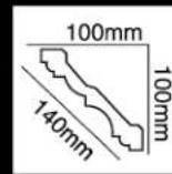
HG-9583 长度(Long):2400mm 面宽(Breath):140mm
