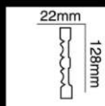
HG-8596 长度(Long):2400mm 面宽(Breath):128mm
