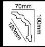
HG-7622 长度(Long):2400mm 面宽(Breath):120mm
