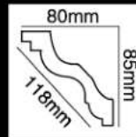
HG-9573 长度(Long):2400mm 面宽(Breath):118mm
