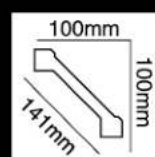
HG-9589 长度(Long):2400mm 面宽(Breath):141mm
