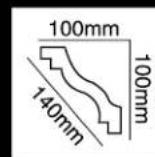
HG-9585 长度(Long):2400mm 面宽(Breath):140mm
