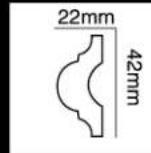
HG-6514 长度(Long):2400mm 面宽(Breath):42mm
