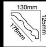
HG-7654 长度(Long):2400mm 面宽(Breath):178mm
