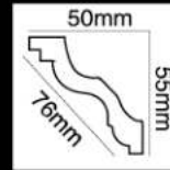
HG-9520 长度(Long):2400mm 面宽(Breath):76mm
